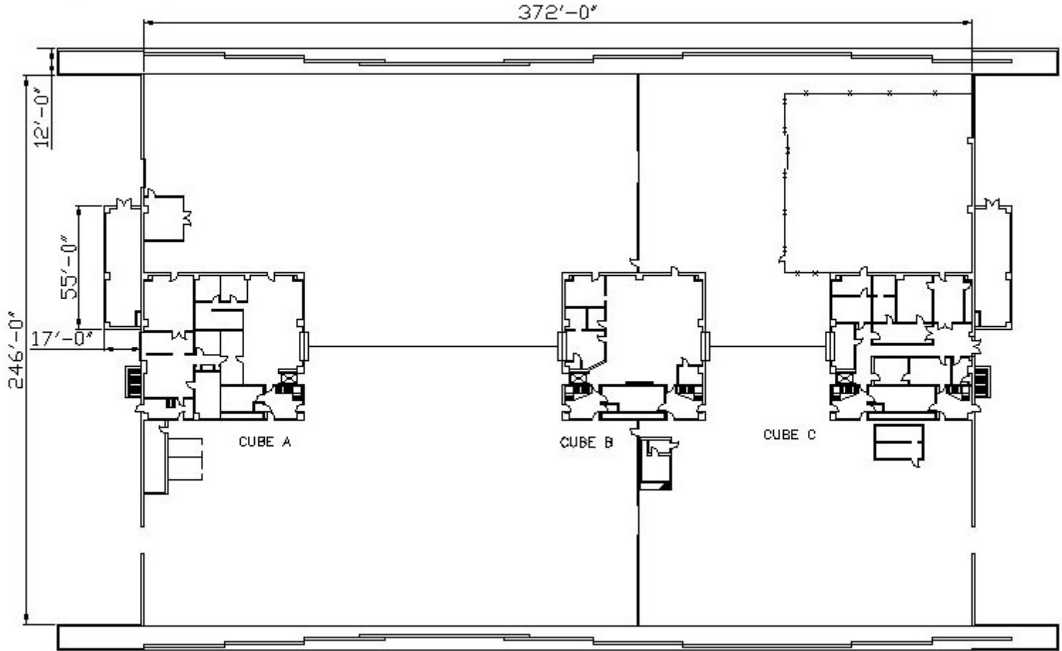
FLOOR PLAN - BLDG 200
